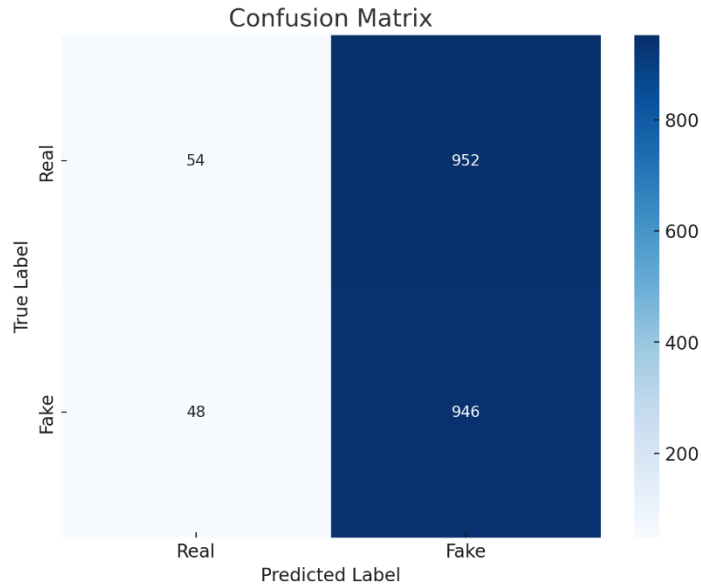
Figure 4: Confusion Matrix for the Testing Set.
